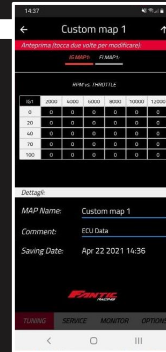
Ignition timing
